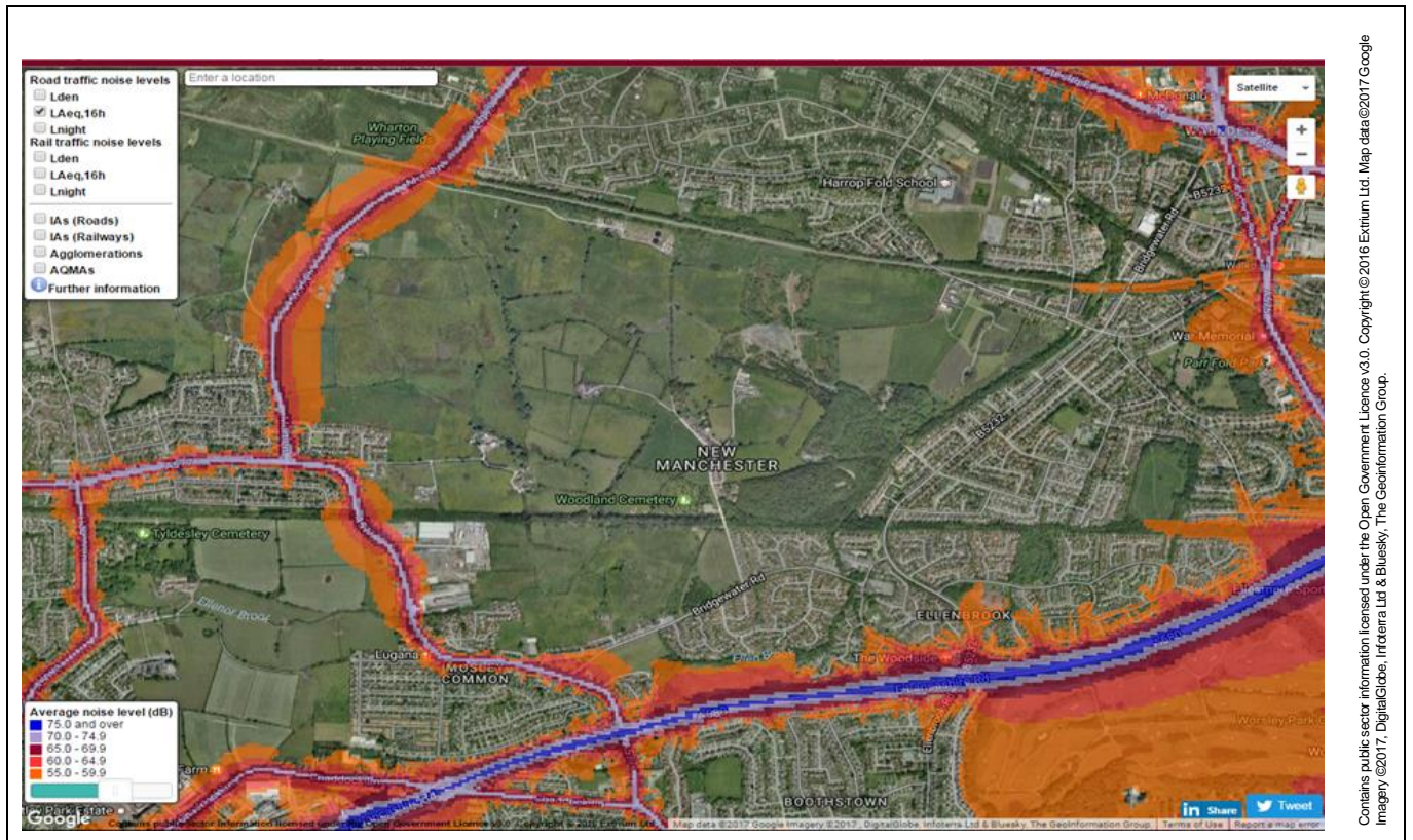
Figure 4 - Average road traffic noise impact
